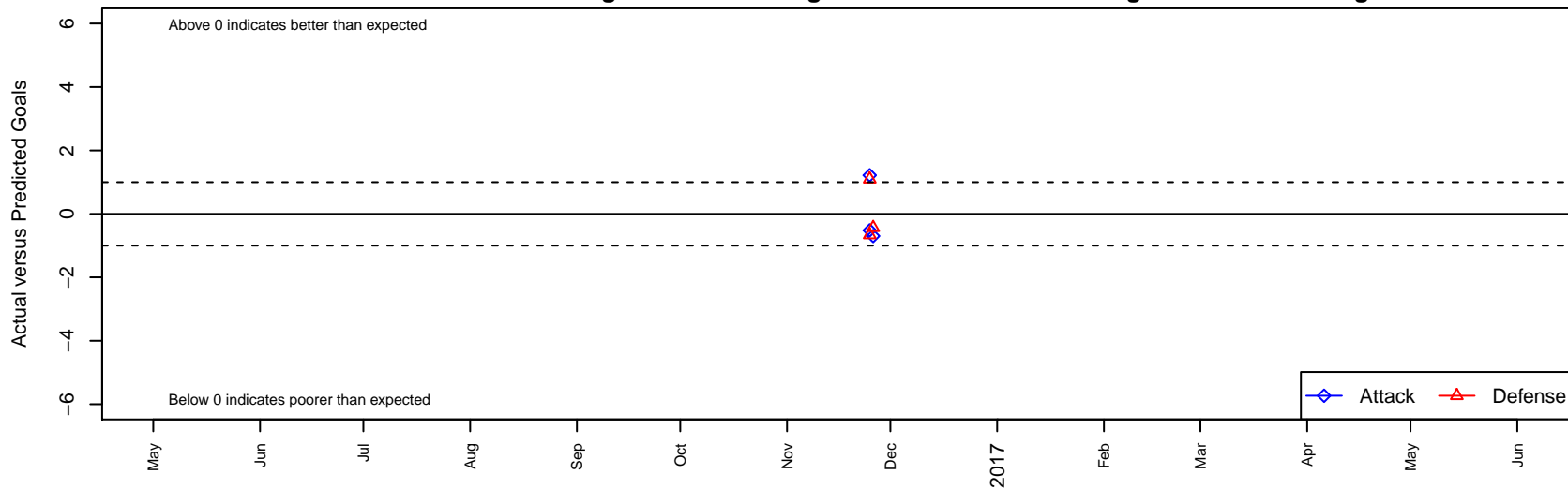
Blue FC Navy B00 Dots are actual minus expected GF (blue circles) and GA (red triangles). Blue line is smoothed change in attack strength. Red is smoothed change in defense strength.
